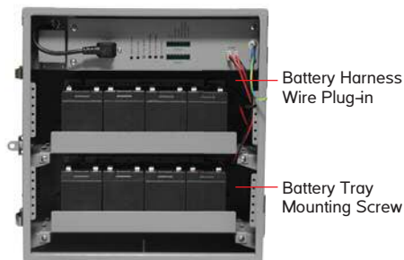
Figure 11: Battery Installation
