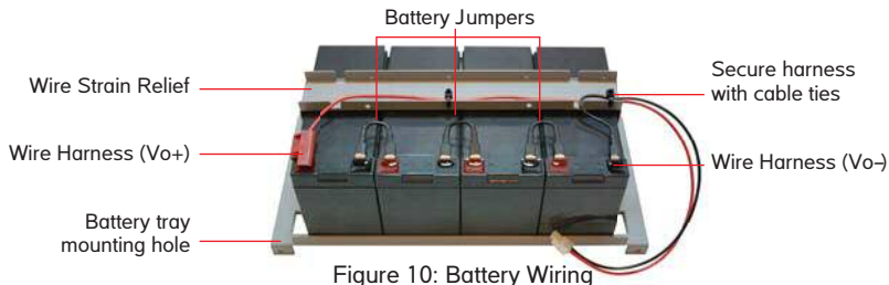
Figure 10: Battery Wiring
