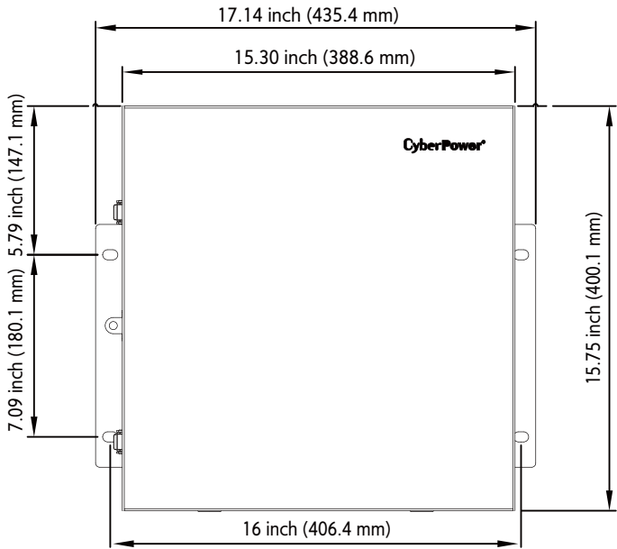
Figure 1: Dimensions (Front View)
